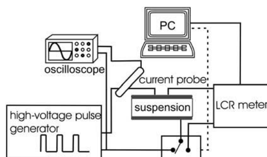
FIGURE 1 A schematic diagram of the system for electroporation and current-voltage and impedance measurements. The cell suspension (100 \mu l) was placed between the electrodes. First, impedance was measured then the system switched electrodes to the high-voltage pulse generator and pulses were delivered. Two to three seconds after the pulses, impedance was measured for the second time and after another 10 s for the third time. For each pulse application, voltage, and current were traced on oscilloscope and stored for further analysis.
